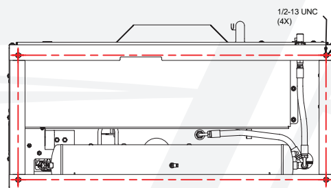
MOUNTING HOLES
